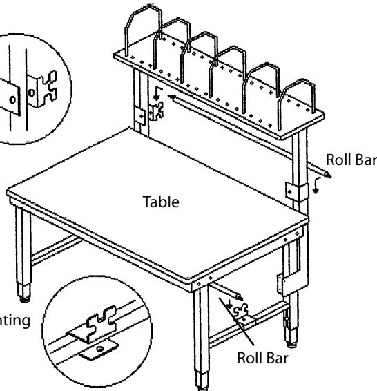
Bracket Mounting ABOVE Table
